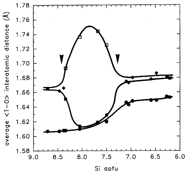
FIGURE 6. Plot of average \langle \text{T-O} \rangle interatomic distances as a function of Si apfu. Midway in the series X-ray structure refinements distinguish three T sites: T_1 (circles), T_2 (open squares), and T_3 (solid squares). Toward each end-member there are only two unique T sites: T_1 and T_2 = T_3 (diamonds). The points of change from three T sites to two are marked by arrows. Data sources are the same as in Figure 4.
