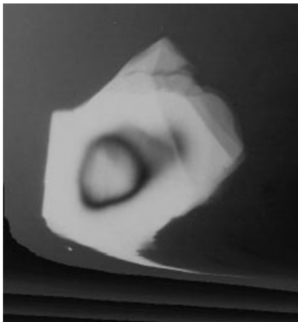
FIGURE 2. Photomicrograph taken with crossed polarizers showing Rb + exchange into a Na-exchanged heulandite at 330 K after 24 h. The diameter of the crystal is approximately 350 \mu\text{m} . The light rim of the crystal shows the Rb-exchanged zone, approximately 96 \mu\text{m} , and the dark boundary indicating that the exchange process had not yet been completed. Note also that the center of the crystal is not at perfect extinction but is a few degrees off. This slightly off-extinction position induces no error in the measurement of t but allows for better visual distinction of the dark boundary.
