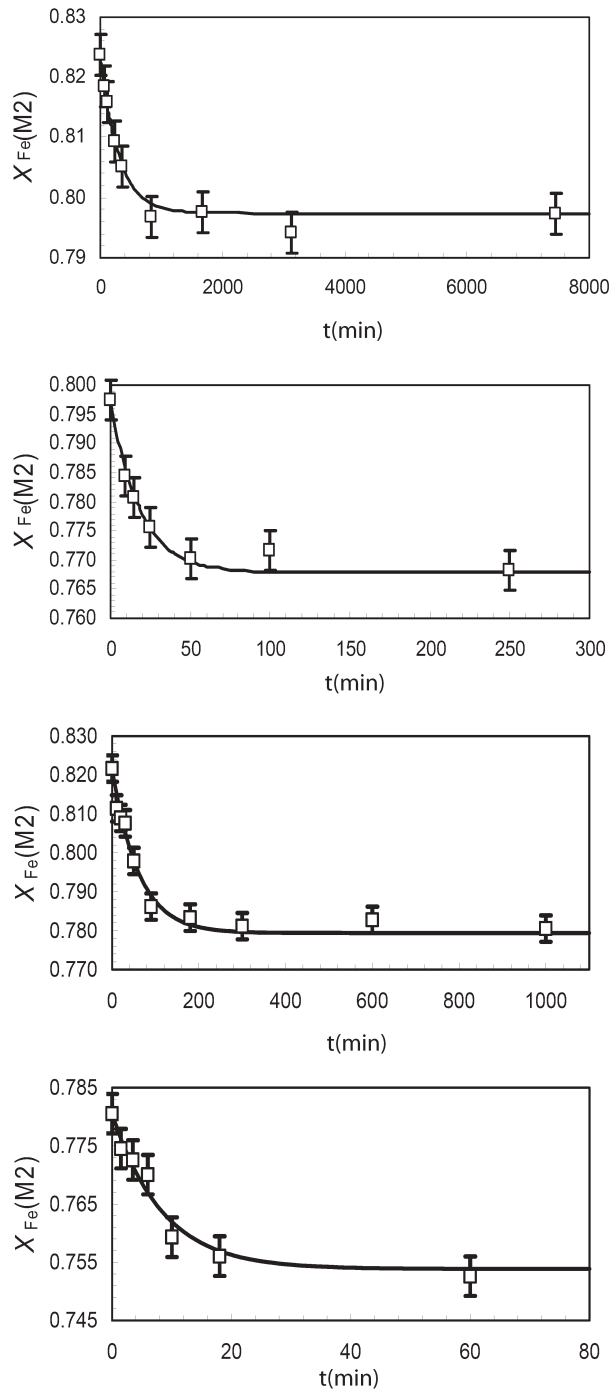
FIGURE 2. Experimental points superimposed on the theoretical curves calculated by Mueller's equation. From top to bottom: annealing at 650, 700, 750, and 800 °C.
