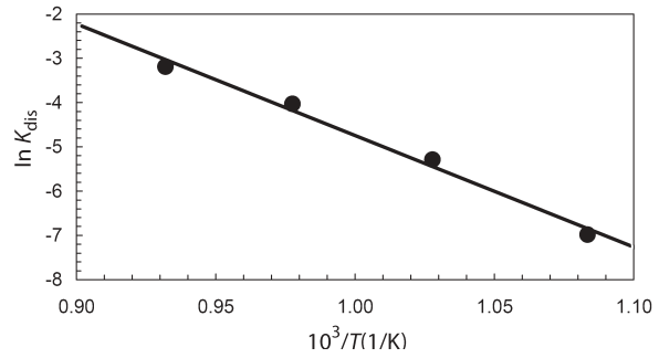
FIGURE 3. Arrhenius plot \ln K_{\text{dis}}^* = \ln K_0 - Q/(RT) which yields an activation energy of 50.03 kcal/mol for the Fe-Mg exchange process for the BTS308 pigeonite sample. The vertical size of the symbols exceeds the uncertainties in \ln K_{\text{dis}}^* . Dashed line: Arrhenius plot obtained by Brizi et al. (2001) for a \text{Wo}_{43}\text{En}_{46}\text{Fs}_{11} augite; dotted line: Arrhenius plot calculated for an orthopyroxene of composition X_{\text{Fe}} = 0.5 using the equation of Ganguly and Tazzoli (1994).
