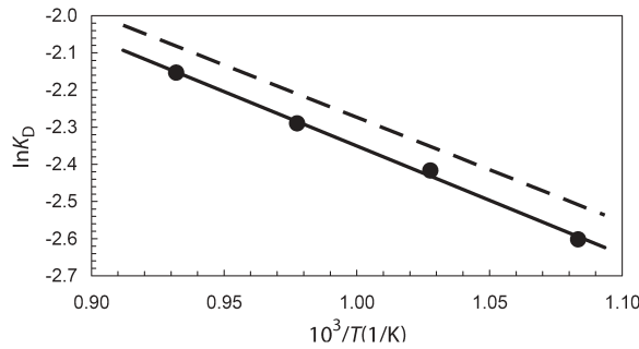
FIGURE 1. A \ln k_D^+ vs. 1/T(K) plot for the BTS308 pigeonite sample. The vertical size of the symbols exceeds the uncertainties in \ln k_D^+ . The dashed line is the calibration by Pasqual et al. (2000).
