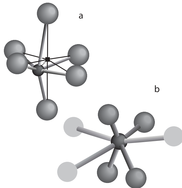
FIGURE 6. (a) Displacement of the cation from the centroid of the M4 site, considered as an octahedron. (b) M4 coordination sphere with the three longest distances subduced, showing the tetrahedral disposition of the four shortest bonds.
