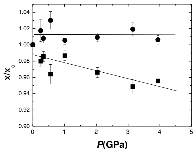
FIGURE 6. Layer thickness (Å) evolution with P (GPa). Full circles = polyhedral layer thickness, full squares = interpolyhedral layer thickness.
