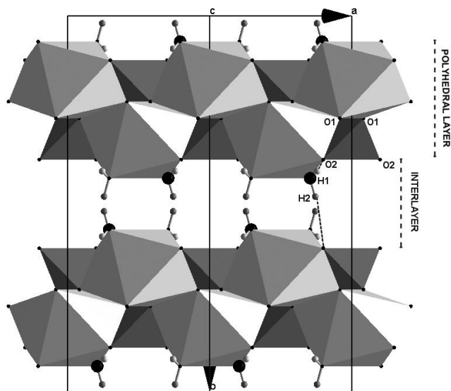
FIGURE 4. Gypsum structure along [001], showing thicknesses of polyhedral and water layers.
