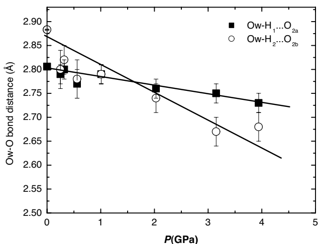
FIGURE 5. Hydrogen bonds (Å) vs. P (GPa).
