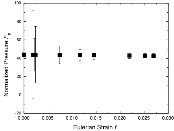
FIGURE 3. Plot of “normalized stress,” defined as F_E = P/[3f_E(1 + 2f_E)^{5/2}] vs. finite strain f_E = [(V_0/V)^{2/3} - 1]/2 . Only values measured before transition, at P lower than 4 GPa, are shown.
