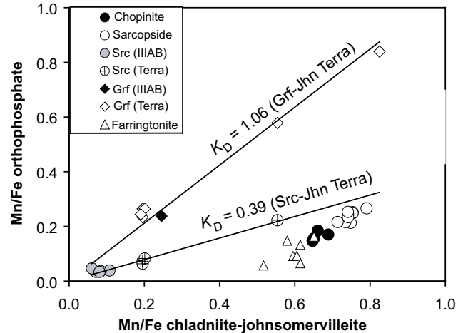
FIGURE 12. Mn/Fe ratios of coexisting chladniite-johnsomervilleite (Jhn), sarcopside (Src)-chopinite, graftonite (Grf) and farringtonite in GRA95209 (this study), terrestrial occurrences (Terra; sources are given in caption for Fig. 11) and IIIAB iron meteorites (Olsen et al. 1999). Lines are least-squares fit to terrestrial graftonite-johnsomervilleite pairs ( R^2 = 0.969 ) and terrestrial sarcopside-johnsomervilleite pairs ( R^2 = 0.986 ).
