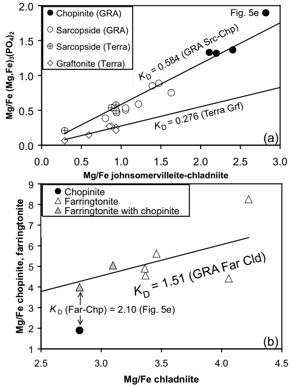
FIGURE 11. Mg/Fe ratios of coexisting chladniite and sarcopside-chopinite in GRA95209 (GRA) and terrestrial (Terra) occurrences (a) and between chladniite and farringtonite in GRA95209 (b). (a) K_D = (\text{Mg/Fe})_{\text{Src}}/(\text{Mg/Fe})_{\text{Cld}} ; R^2 = 0.936 for least-squares fit to sarcopside-chopinite (GRA95209 data only) and K_D = (\text{Mg/Fe})_{\text{Grf}}/(\text{Mg/Fe})_{\text{Cld}} ; R^2 = 0.858 for least-squares fit to terrestrial graftonite. (b) The two points give K_D (\text{Far-Chp}) = (\text{Mg/Fe})_{\text{Far}}/(\text{Mg/Fe})_{\text{Chp}} from analytical data on grains analyzed in PTS ,39 area 2-1 (Fig. 5e) and the line gives a least-squares fit for all the farringtonite data: K_D = (\text{Mg/Fe})_{\text{Far}}/(\text{Mg/Fe})_{\text{Cld}} ; R^2 = 0.411 . Chopinite in the second 3-phase assemblage did not give a satisfactory analysis, and so is not plotted. Sources for terrestrial pairs: Corbella i Cordoní and Malgarejo i Draper (1990), Černý et al. (1998), Livingstone (1980), Roda et al. (2004), F. Hatert (personal communication 2007); for GRA95209 (this study).
