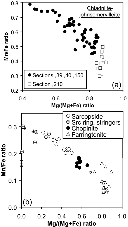
FIGURE 8. (a) Variation of Mn/Fe ratio with X Mg = Mg/(Mg+Fe) ratio in chladniite-johnsomervilleite. (b) Variation of Mn/Fe ratio with X Mg = Mg/(Mg+Fe) ratio in orthophosphates in PTS, 39 and 40 and PS, 150. Ring and stringers of sarcopside (Src) occur in the metal sheet in PS, 150 (e.g., Fig. 6b). The identity of one composition (queried farringtonite) is richer in Fe than other farringtonite. Sources of data: Floss (1999); T. McCoy (personal communication 2005); McCoy et al. (2006); this study.
