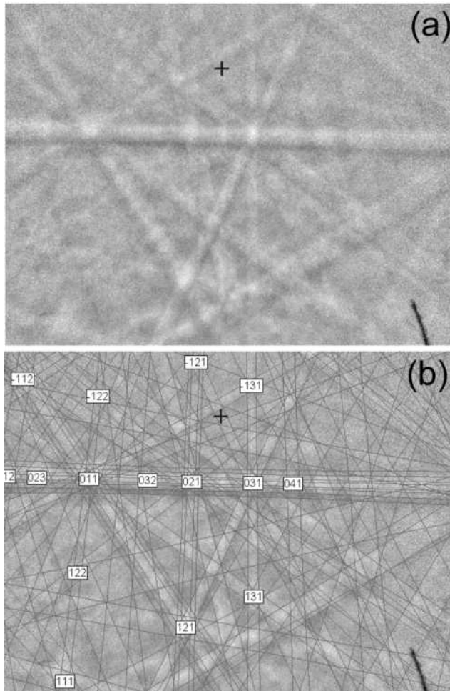
FIGURE 2. (a) Kikuchi pattern for chopinite section PTS ,40, area 1-2a. The numbers on the image are Miller indices for the poles at the intersection of the bands, which are produced by specific sets of crystallographic planes. The mean angular deviations for the match (b) are 0.536. The + in both images is an artifact of the calibration (basically pattern centering).
