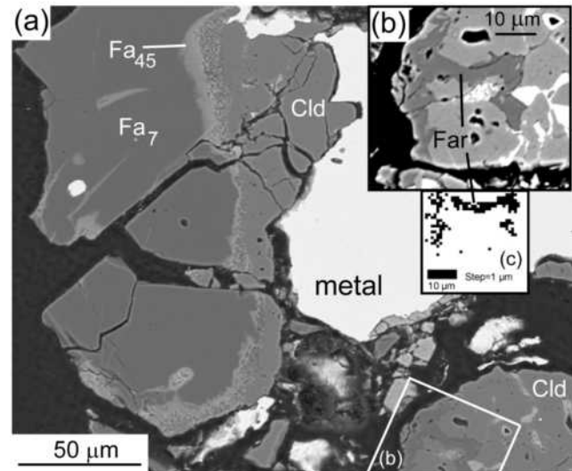
FIGURE 3. Back-scattered electron (BSE) images of fayalitic rims on forsterite in GRA95209, PTS ,40, area 4 (Table 2). Speckled band between fayalitic rim and chladniite is a mixture of fayalitic olivine and silica (identification using energy dispersive spectroscopy). Dark areas are epoxy exposed by fragmentation of the section. (b) Contrast-enhanced, brightened, and enlarged portion of BSE image enclosed in white frame in a to bring out M-shaped area of farringtonite (Table 6). (c) Map of the M-shaped area of farringtonite obtained by electron backscatter diffraction (Table 1 for area 4-1) using only points with MAD < 1 (all farringtonite, pixels plotted as black squares). The white area of the map includes pixels from matches with MAD > 1 (Table 1) and pixels for which no match could be found among the phases listed in Table 1. Cld = chladniite, Fa = fayalite content of forsterite (in mole percent from electron microprobe analysis), Far = farringtonite.
