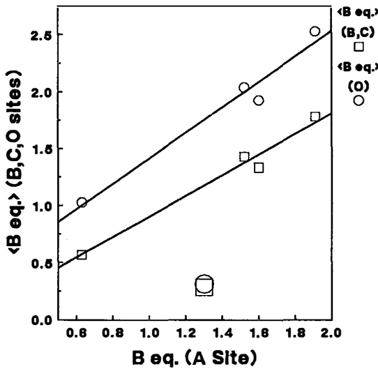
FIG. 6. Mean equivalent isotropic displacement-factor for the B and C cationic sites (squares) and oxygen sites (circles) versus that for the A site for all refined structures of wodginite. Data for sample TSE-76 are necessarily excluded, as displacement parameters were not refined for this structure. Symbol coding is as in Figure 3.
