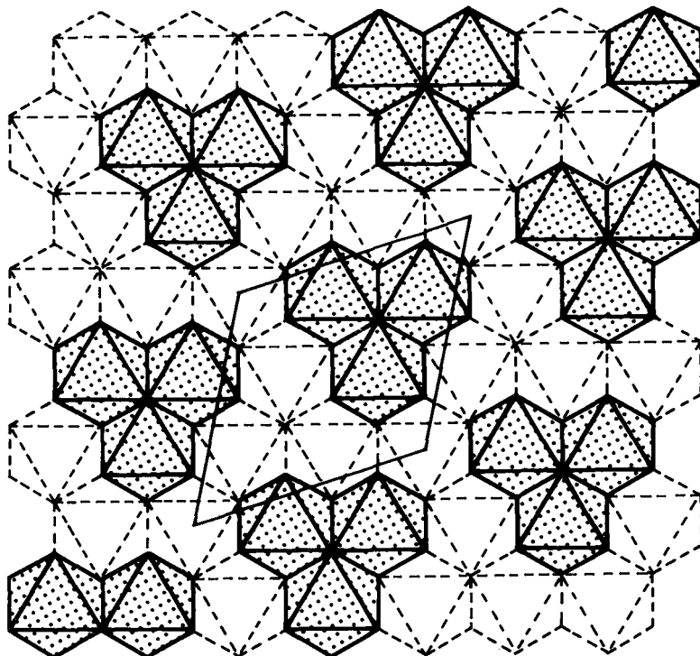
FIG. 2. The ideal structure of simpsonite, as projected along Z . Solid lines represent polyhedra of one level, and broken lines, those of adjacent levels. Ta-bearing polyhedra are shaded; Al-bearing polyhedra are unshaded. One unit cell is two layers of polyhedra deep; the outline of one unit cell is shown in fine rule.
