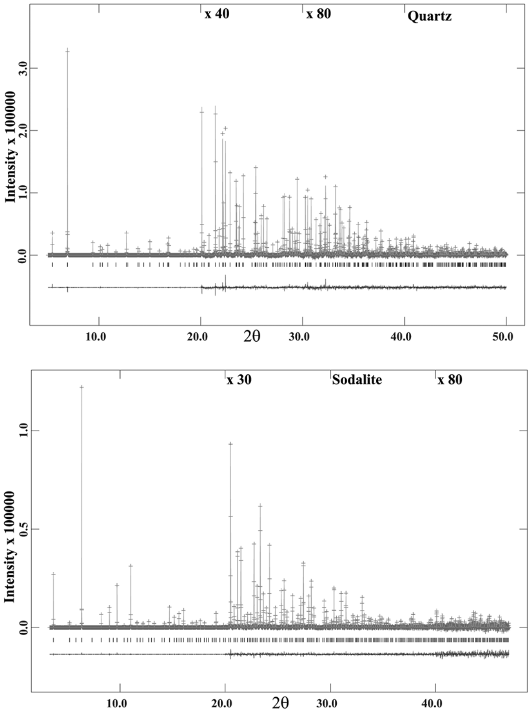
FIG. 1. HRPXRD traces for (a) quartz, (b) sodalite, (c) tremolite, and (d) meionite Me_{79.6} , together with the calculated (continuous line) and observed (crosses) profiles. The difference curve ( I_{obs} - I_{calc} ) is shown at the bottom. The short vertical
