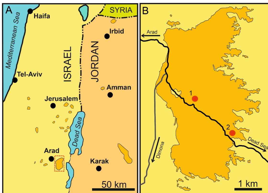
Figure 1. (A) Schematic map of the Middle East with outcrops of Hatrurim Complex (dark-yellow). The framed part is magnified in B. (B) Schematic map of the Hatrurim Basin. The sampling places of rankinite paralavas are marked by red circles—1. Gurim Anticline, 2. Zuk Tamrur (modified after Reference [20]).
