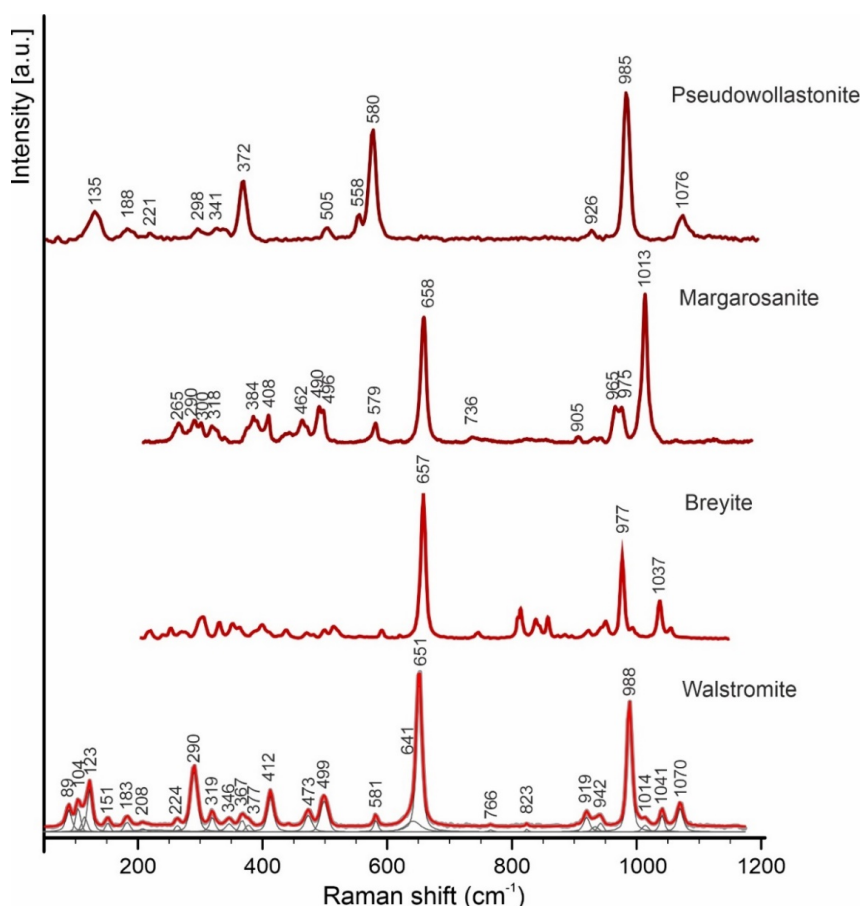
Figure 4. Raman spectra of walstromite from paralava of the Gurim Anticline and breyite (Anzoloni et al., 2018 [16], excitation line 532 nm), margarosanite from Parker shaft, Franklin, NJ, USA (RRUFF, 532 nm) and pseudowollastonite-2M from gehlenite hornfels of the Negev Desert (488 nm).
