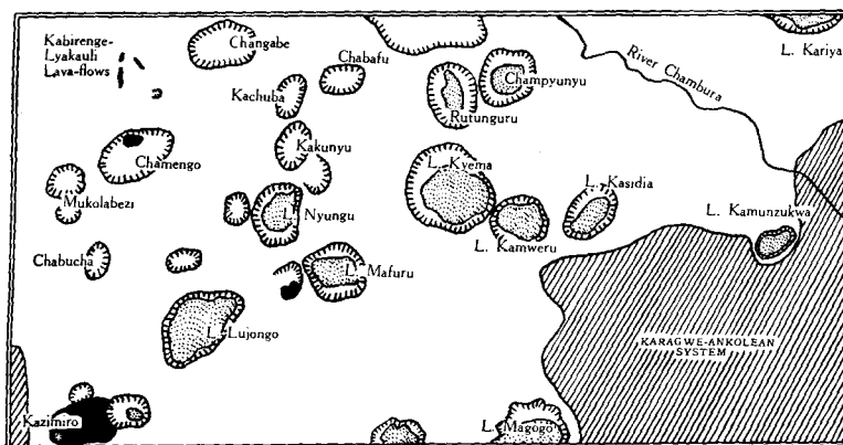
FIG. 1. Sketch-map showing the explosion craters and lava occurrences of part of the Bunyaruguru volcanic field of south-west Uganda. The area illustrated is 7\frac{1}{2} by 3\frac{1}{4} miles. Topographical and geological details from an unpublished field map by A. D. Combe, Geological Survey of Uganda.
