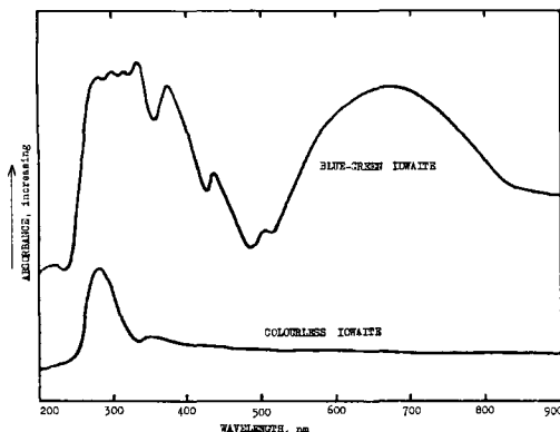
FIG. 1. Electronic absorption spectra of iowaites, viewed along the optic axis ( c ).
