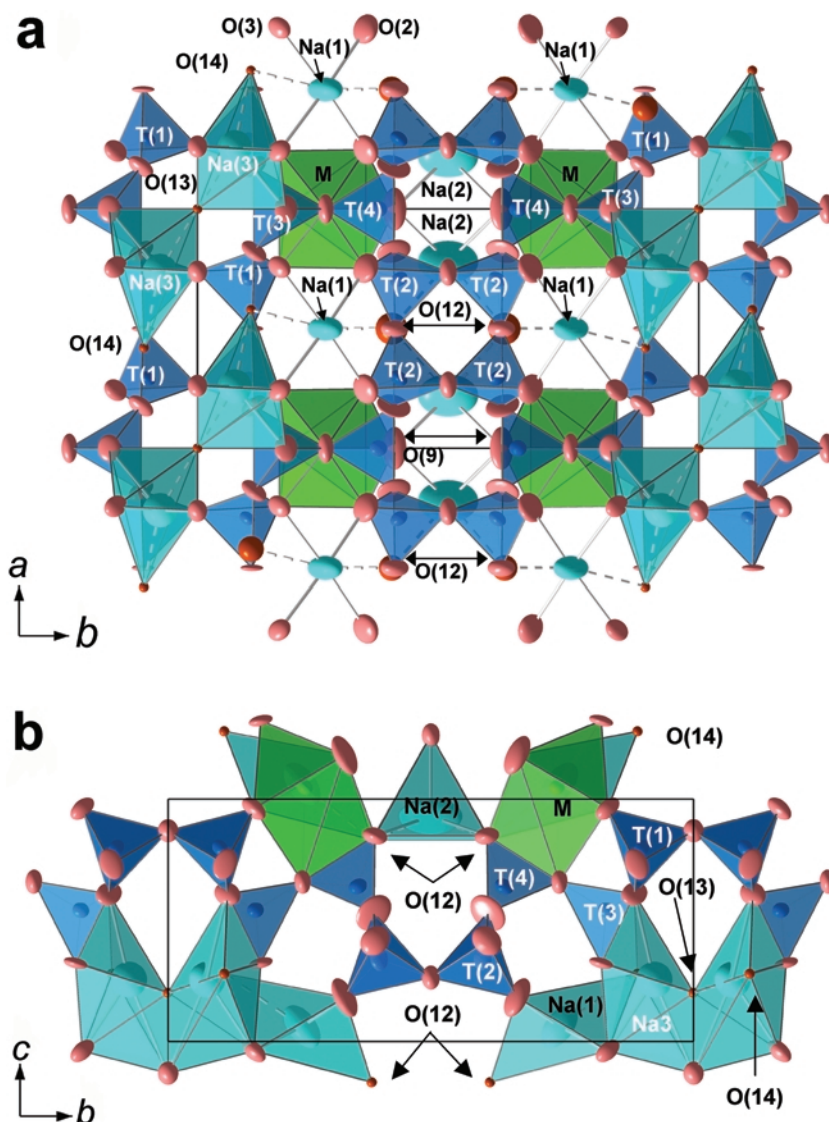
FIG. 5. Projection of the sazhinite structure (a) onto (001) and (b) onto (100). In (a) the Na(1) and Na(2) sites and coordinating O atoms are shown as ellipsoids at 95% probability. In both figures the O(12), O(13) and O(14) O atoms are shown as spheres.
