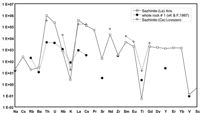
FIG. 7. Chondrite-normalized pattern of crystal 1 (point A = open squares). Whole-rock composition of Aris phonolite (von Knorring and Franke, 1987; filled dots) and data for sazhinite (Ce) Lovozero (Es'kova et al. , 1974) (grey diamonds).
