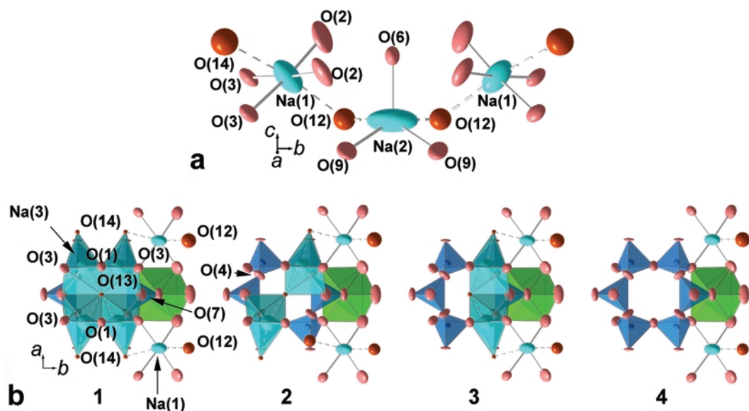
FIG. 6. The local bonding environments for the (a) Na(1) and Na(2) sites and (b) the Na(3) sites. In (b) different local configurations for the Na(3) site are shown: while configuration 1 is not allowed because of very short Na(3)–Na(3) distances (2.31 Å); all the other cases are possible.
