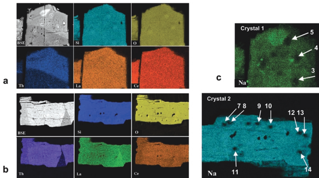
FIG. 3. Back-scattered electron (BSE) images and X-ray maps of (a) crystal 1 and (b) crystal 2. (c) Na X-ray maps of crystals 1 and 2 showing beam damage after EMP analysis.
